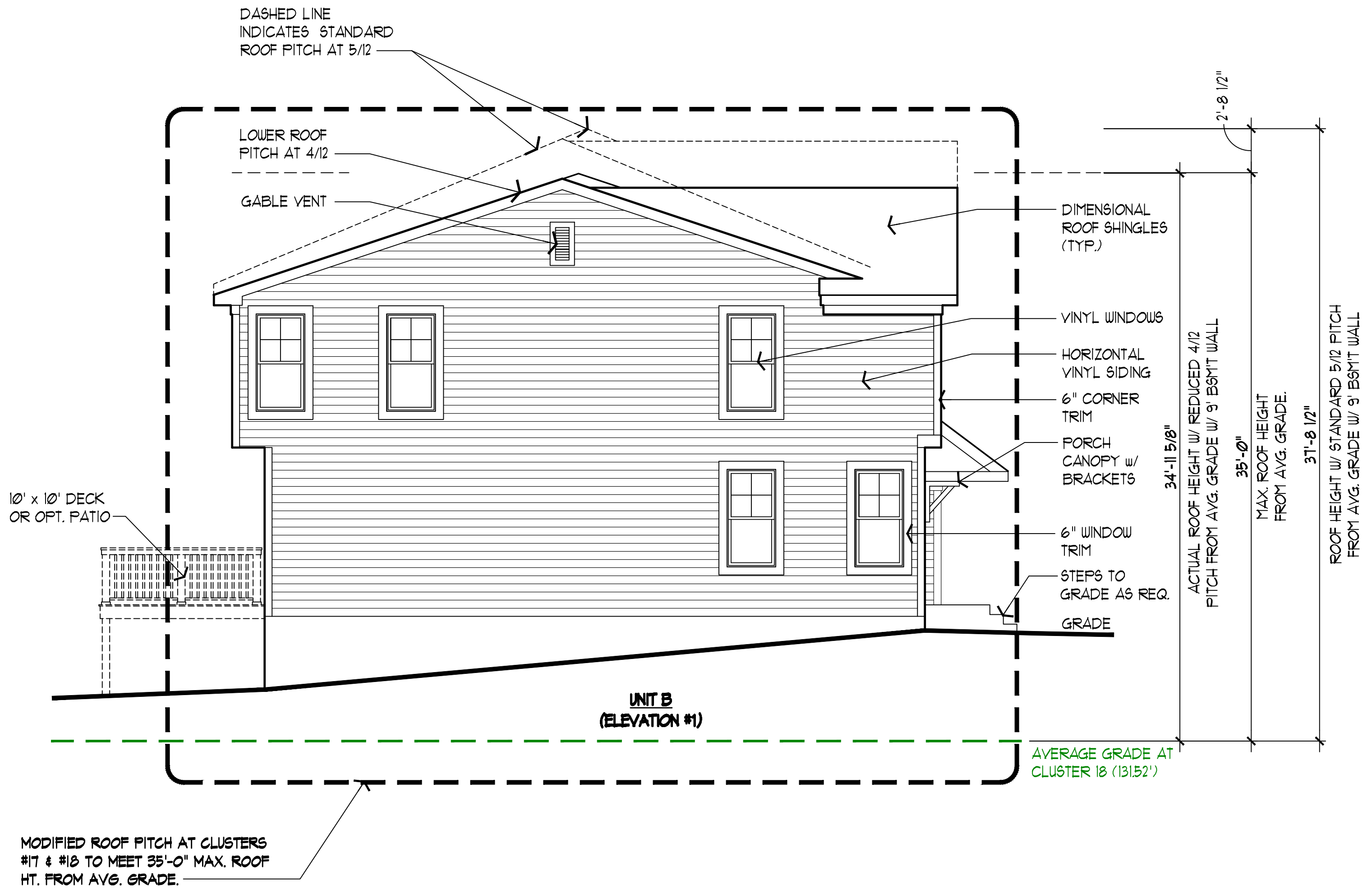
LEFT SIDE ELEVATION (10-UNIT BUILDING)
